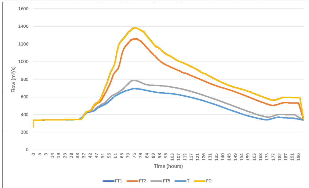
Plate 3.2 – Humber EWL model fluvial inflows on the River Ouse
