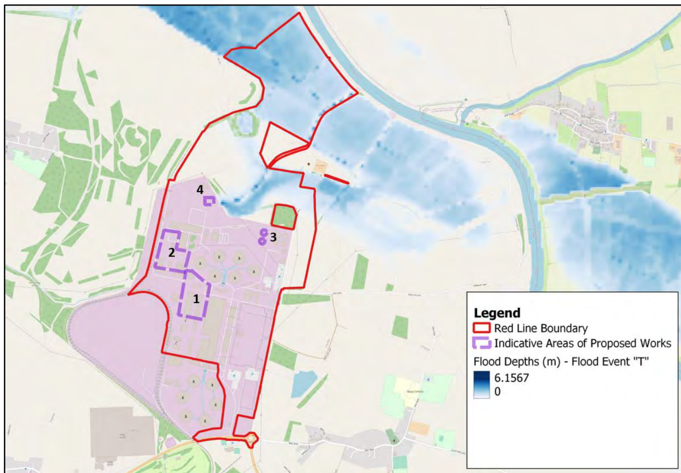
Figure 1 – Flood Depths defended future day scenario (2046H) – Flood Event “T”
