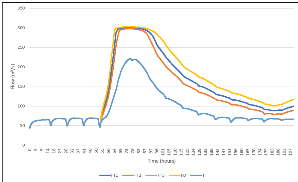
Plate 3.4 – Humber EWL model fluvial inflows on the River Don
