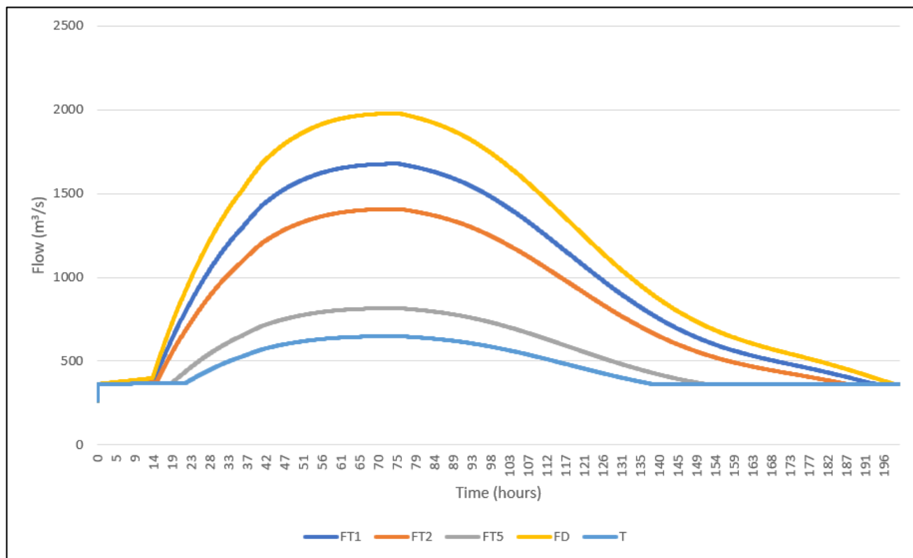
Plate 3.5 – Humber EWL model fluvial inflows on the River Trent
