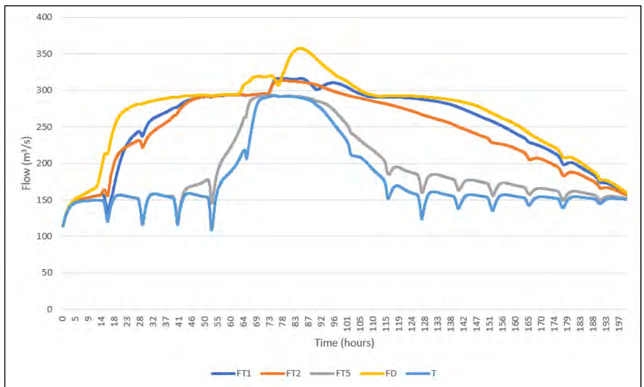
Plate 3.3 – Humber EWL model fluvial inflows on the River Aire
